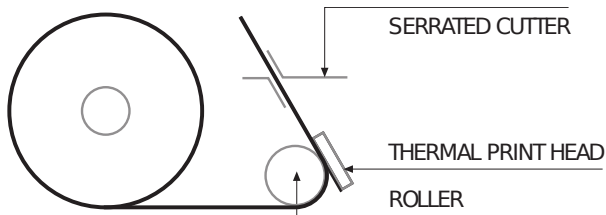
Figure 1 Printer Mechanism
